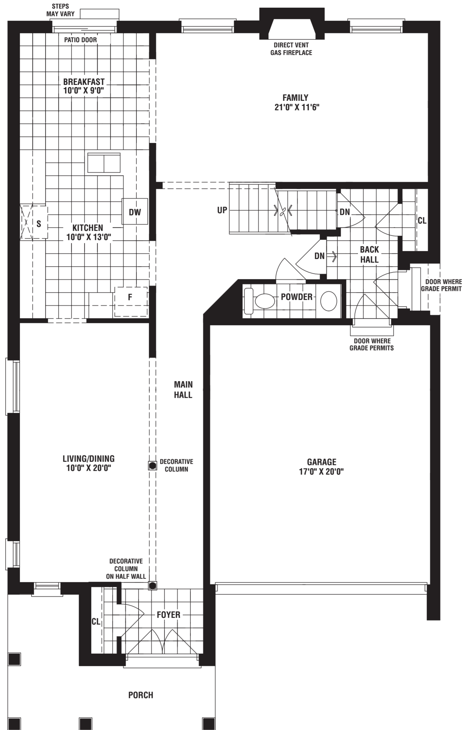
GROUND FLOOR ELEV. 'A', 'B', 'C'
