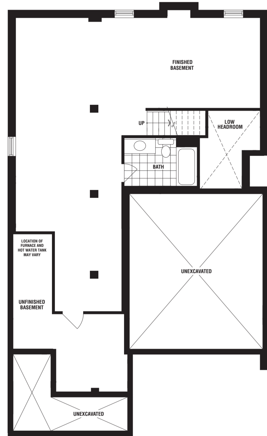
BASEMENT PLAN ELEV. 'A', 'B', 'C'
