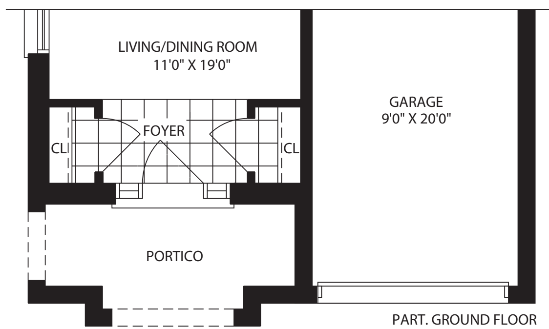
PART. GROUND FLOOR ELEV. 'B'
