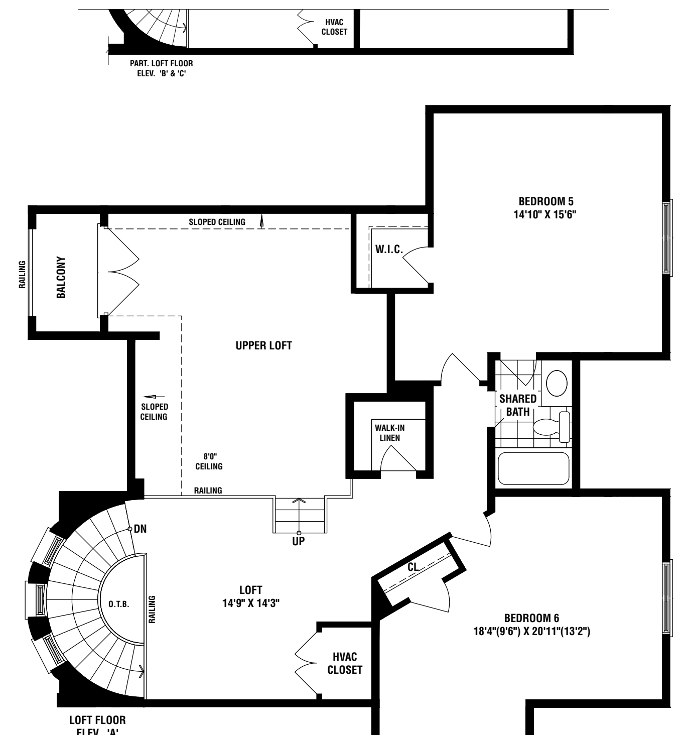
LOFT FLOOR ELEV. 'A'
