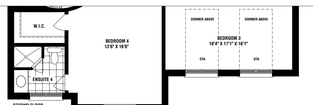
SECOND FLOOR ELEV. 'C'
