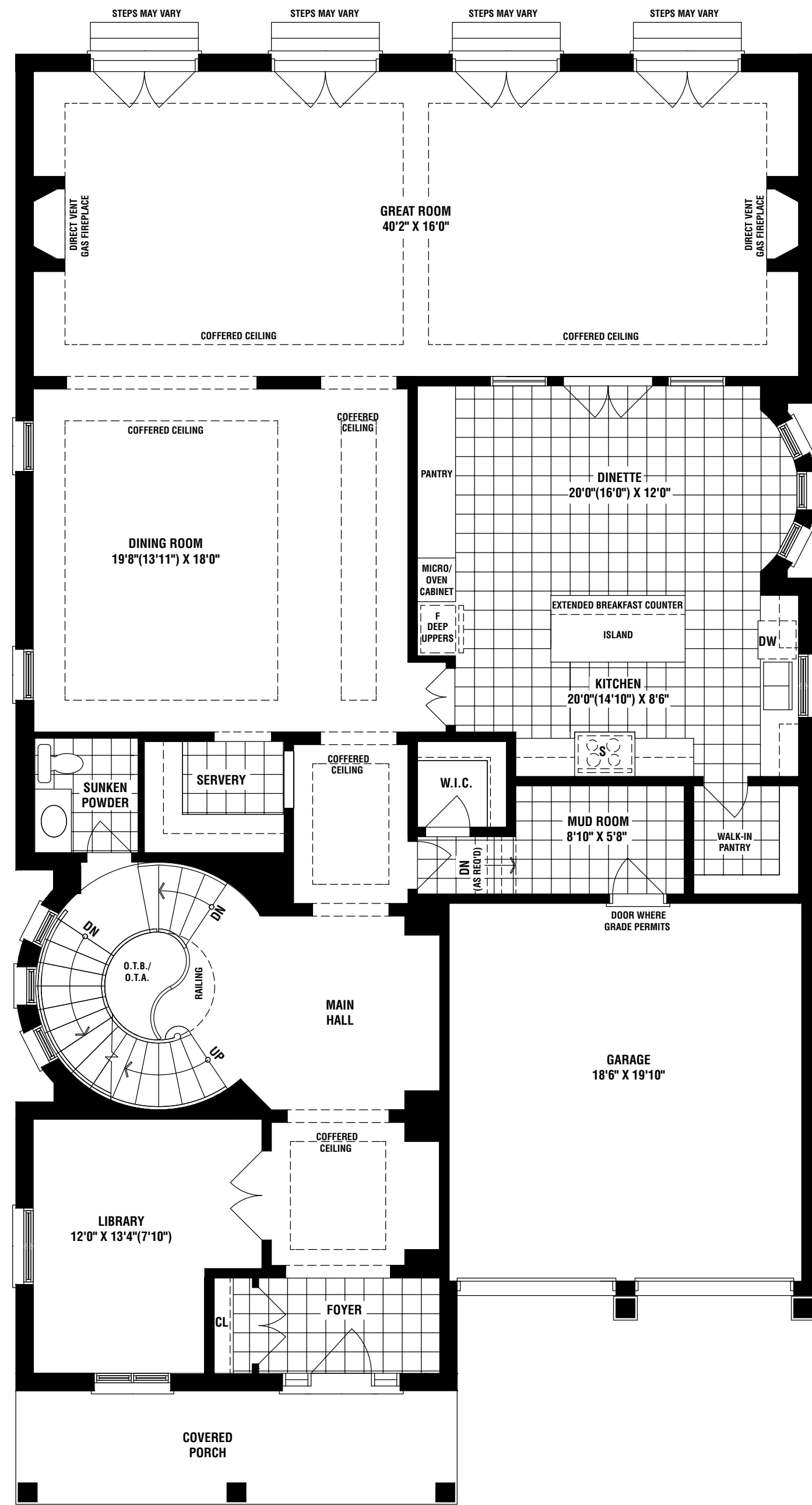
GROUND FLOOR ELEV. 'A'
