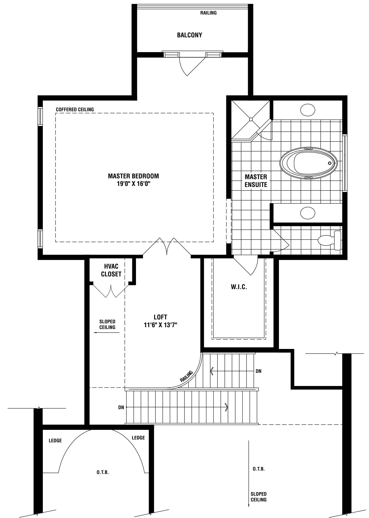
LOFT FLOOR PLAN ELEV. 'A'
