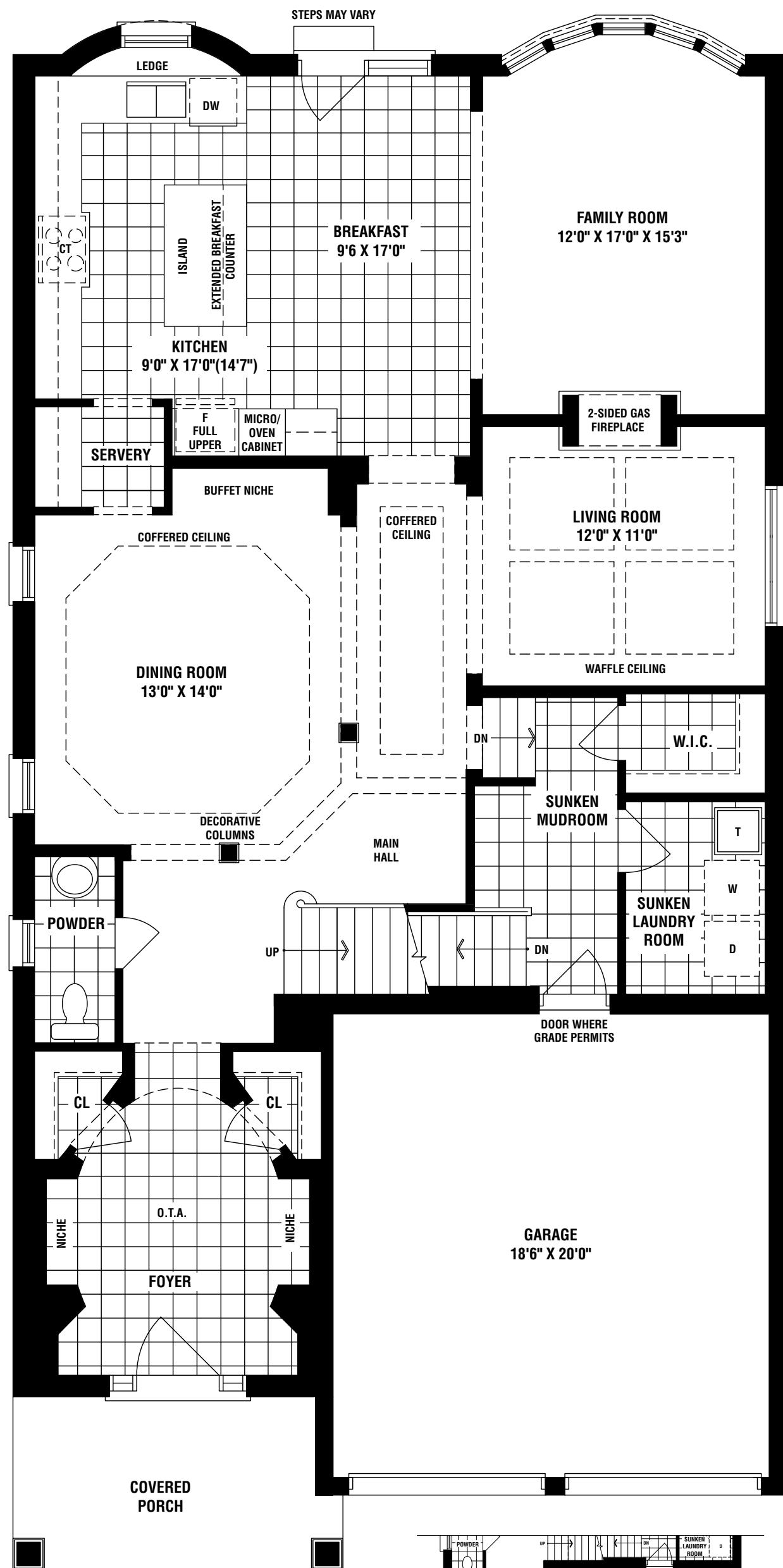
GROUND FLOOR PLAN ELEV. 'A'
