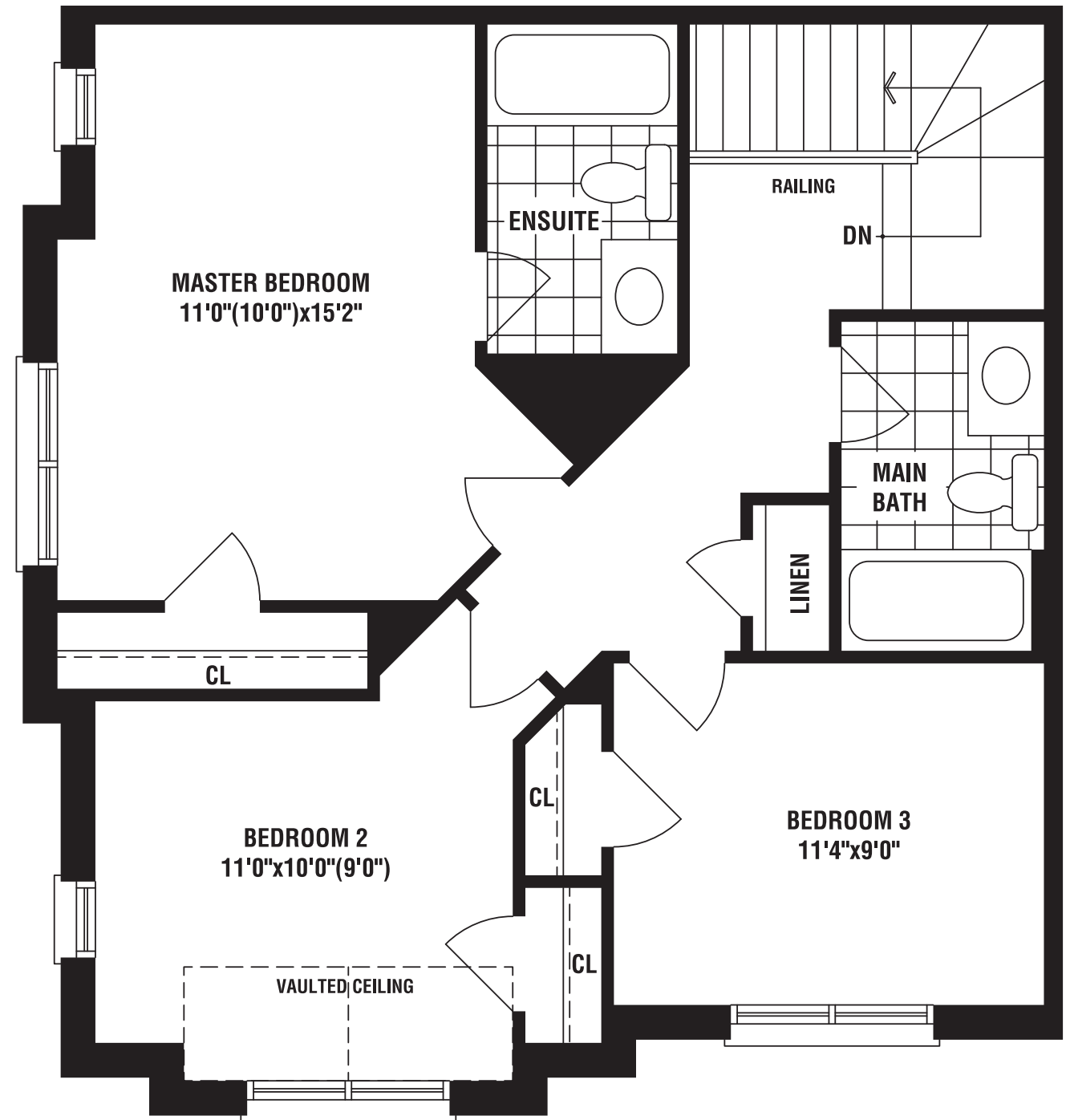
THIRD FLOOR ELEV. 'A'
