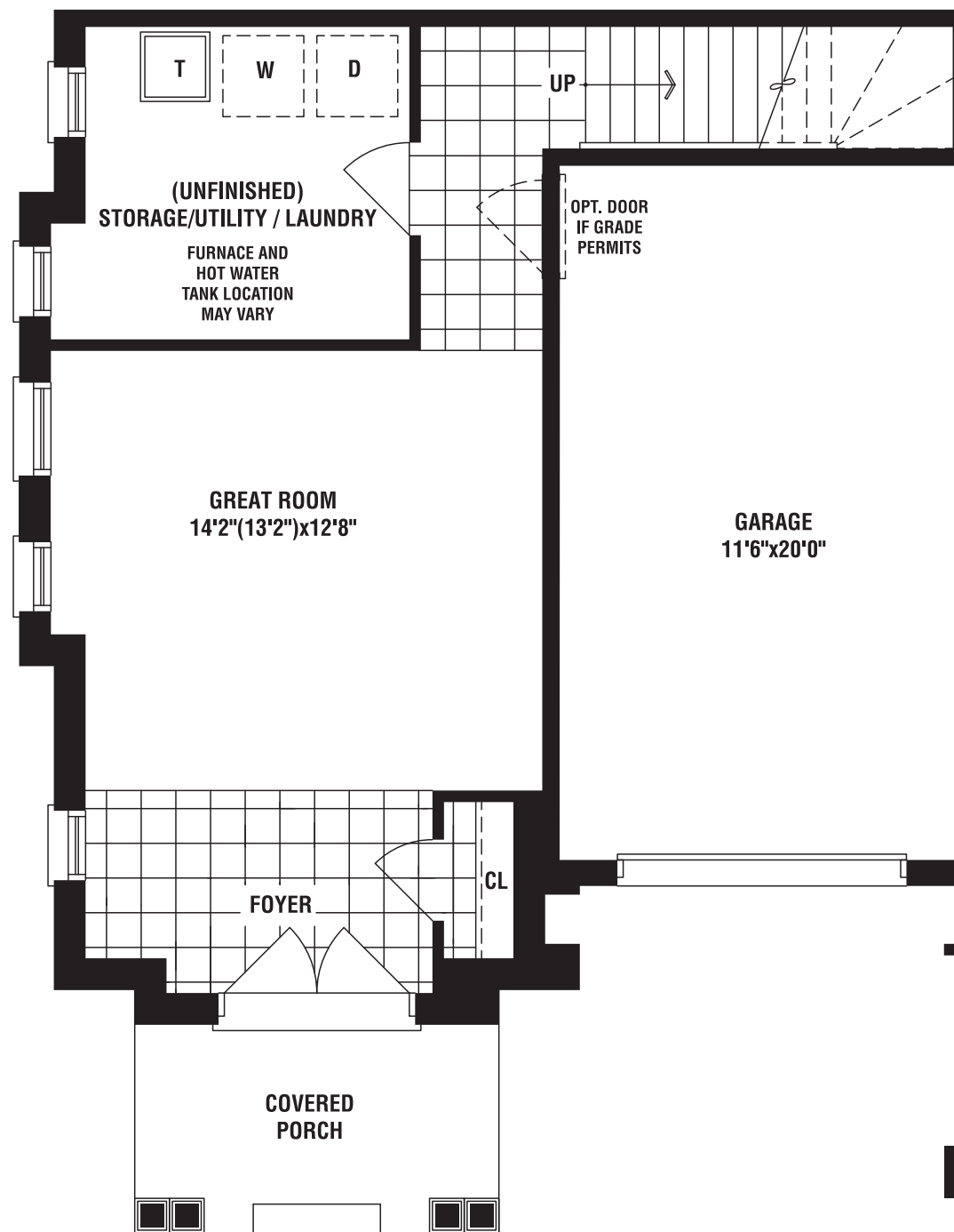
GROUND FLOOR ELEV. 'A'
